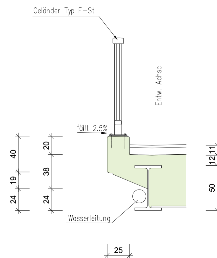
Detail A Randbalken M 1:25
